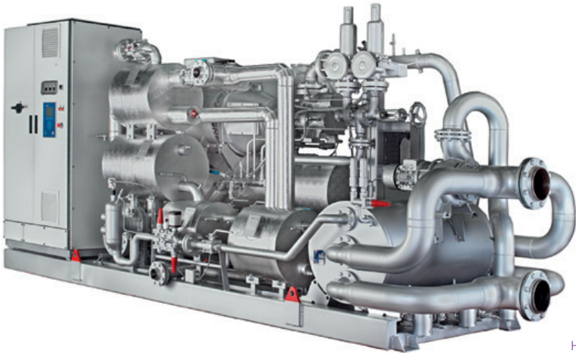
HeatPAC 157 HR
